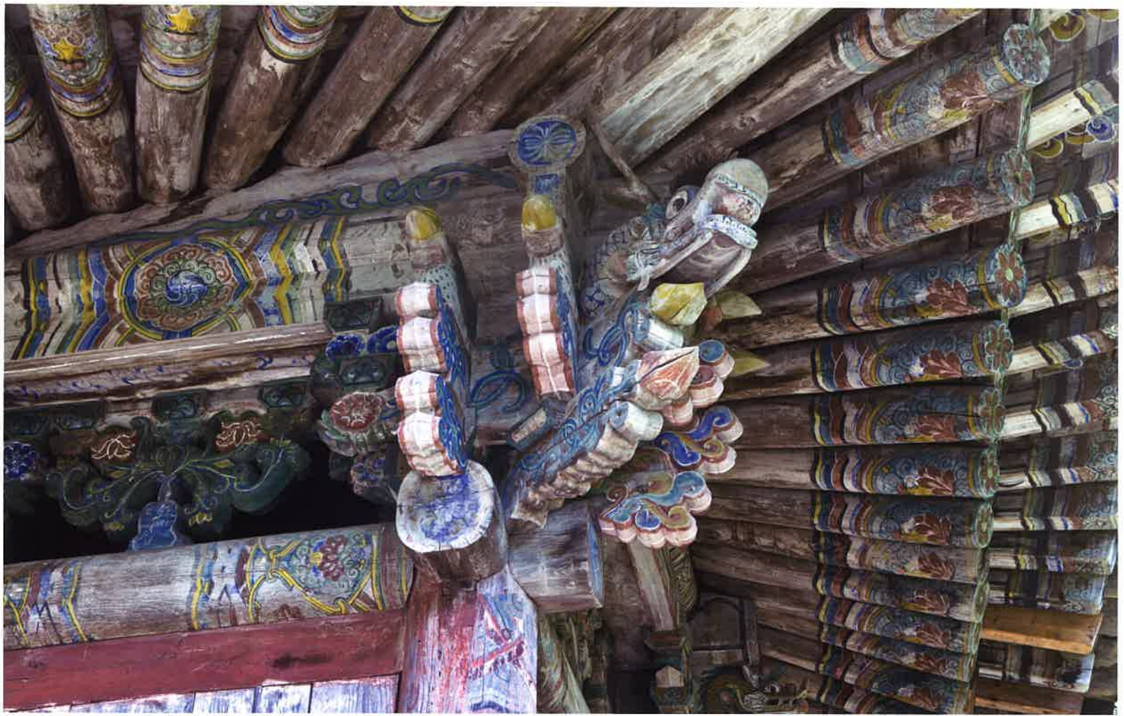
불지암 앞면 동쪽 귀포 / 佛地庵 前面 東側 耳包 / front eastern corner brackets, Puljiam
