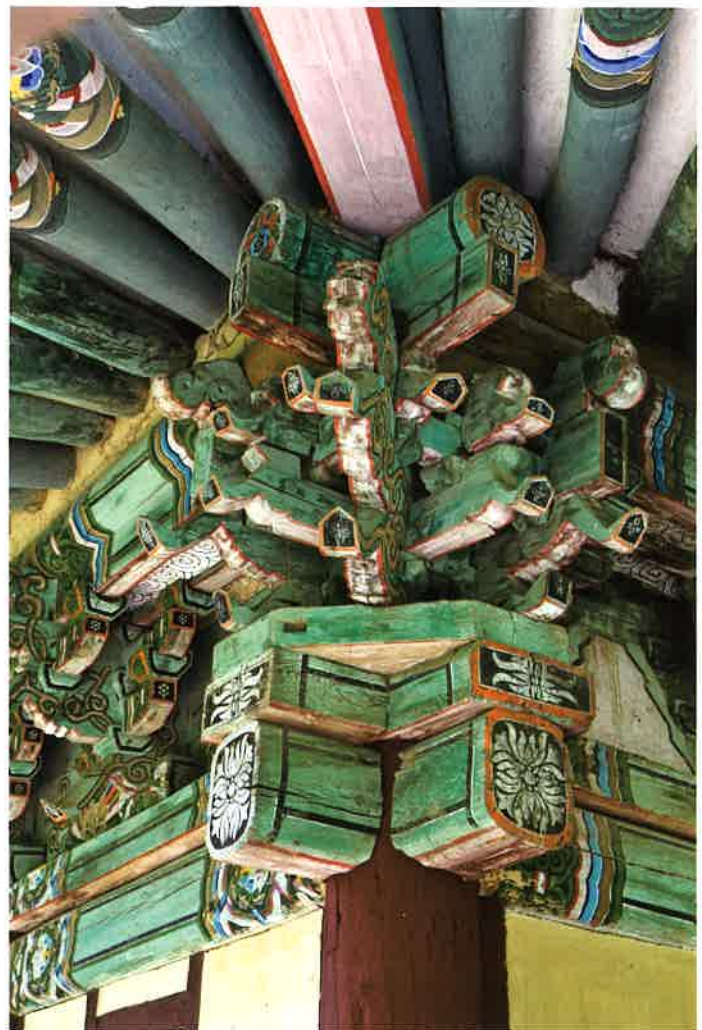
불지암 뒷면 귀포 / 佛地庵 後面 耳包 backward corner brackets, Puljiam
