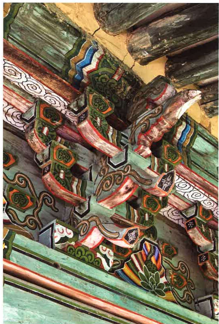
불지암 동쪽 측면 주간포 / 佛地庵 東側 柱間包 eastern brackets between columns, Puljiam
