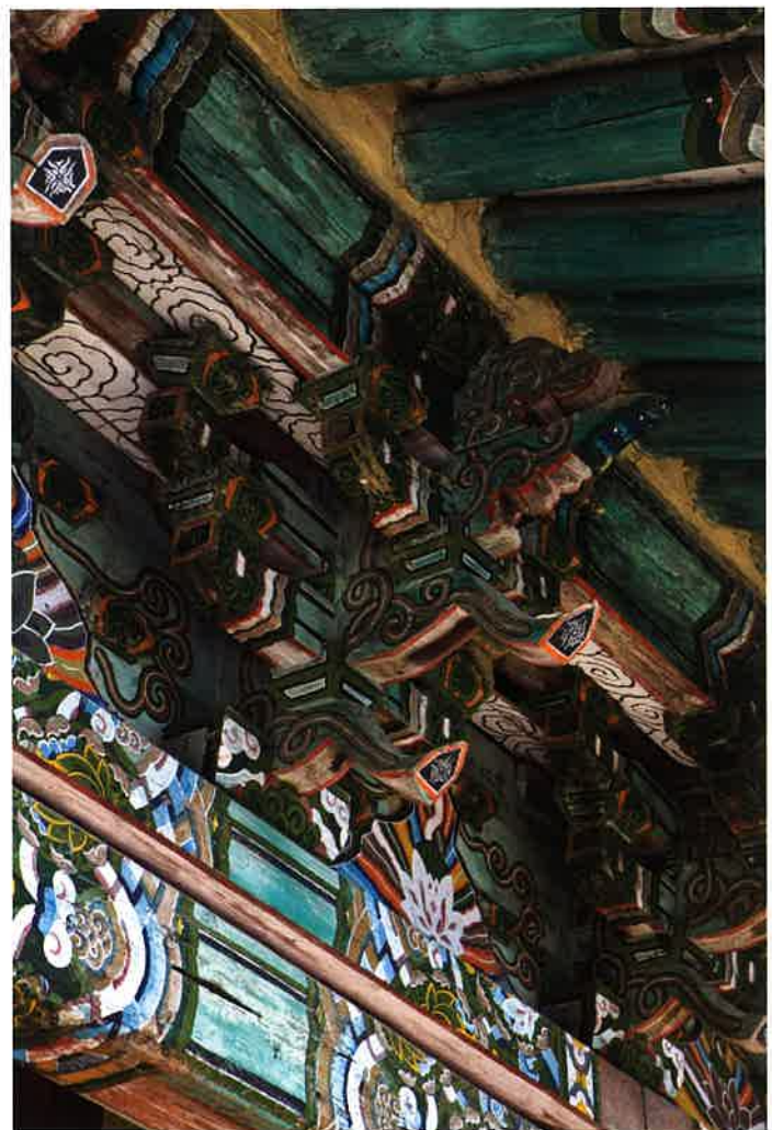
불지암 앞면 주간포 / 佛地庵 前面 柱間包 brackets between front columns, Puljiam
